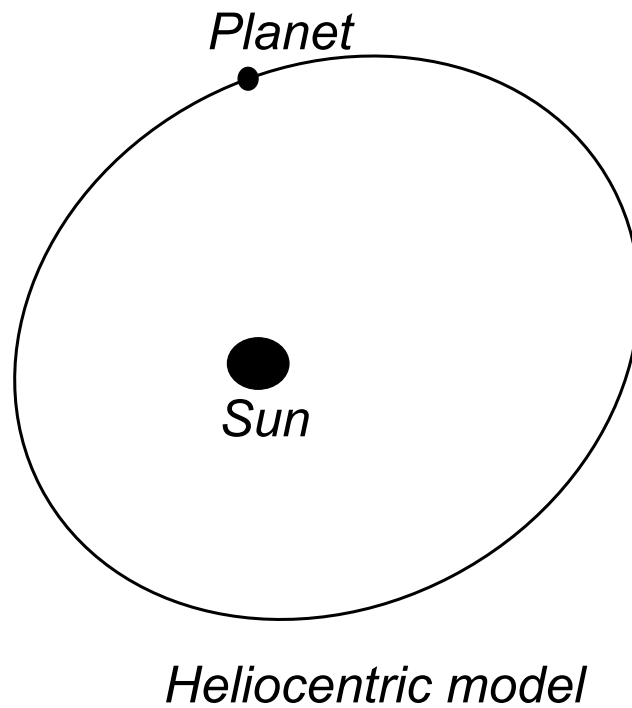
Figure 6: Heliocentric model
